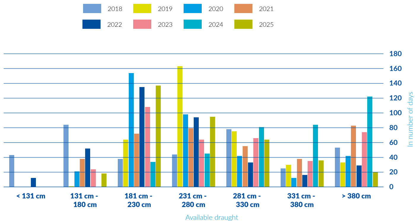
FIGURE 2: NUMBER OF DAYS PER YEAR FOR AVAILABLE DRAUGHT INTERVALS AT KAUB
