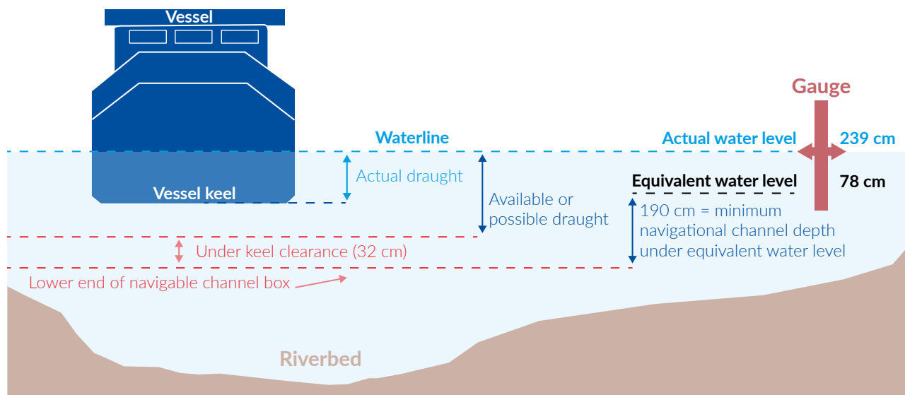
FIGURE 1: ACTUAL WATER LEVEL, ACTUAL DRAUGHT, EQUIVALENT WATER LEVEL, MINIMUM NAVIGATION CHANNEL DEPTH AND POSSIBLE OR AVAILABLE DRAUGHT AT KAUB/MIDDLE RHINE *
